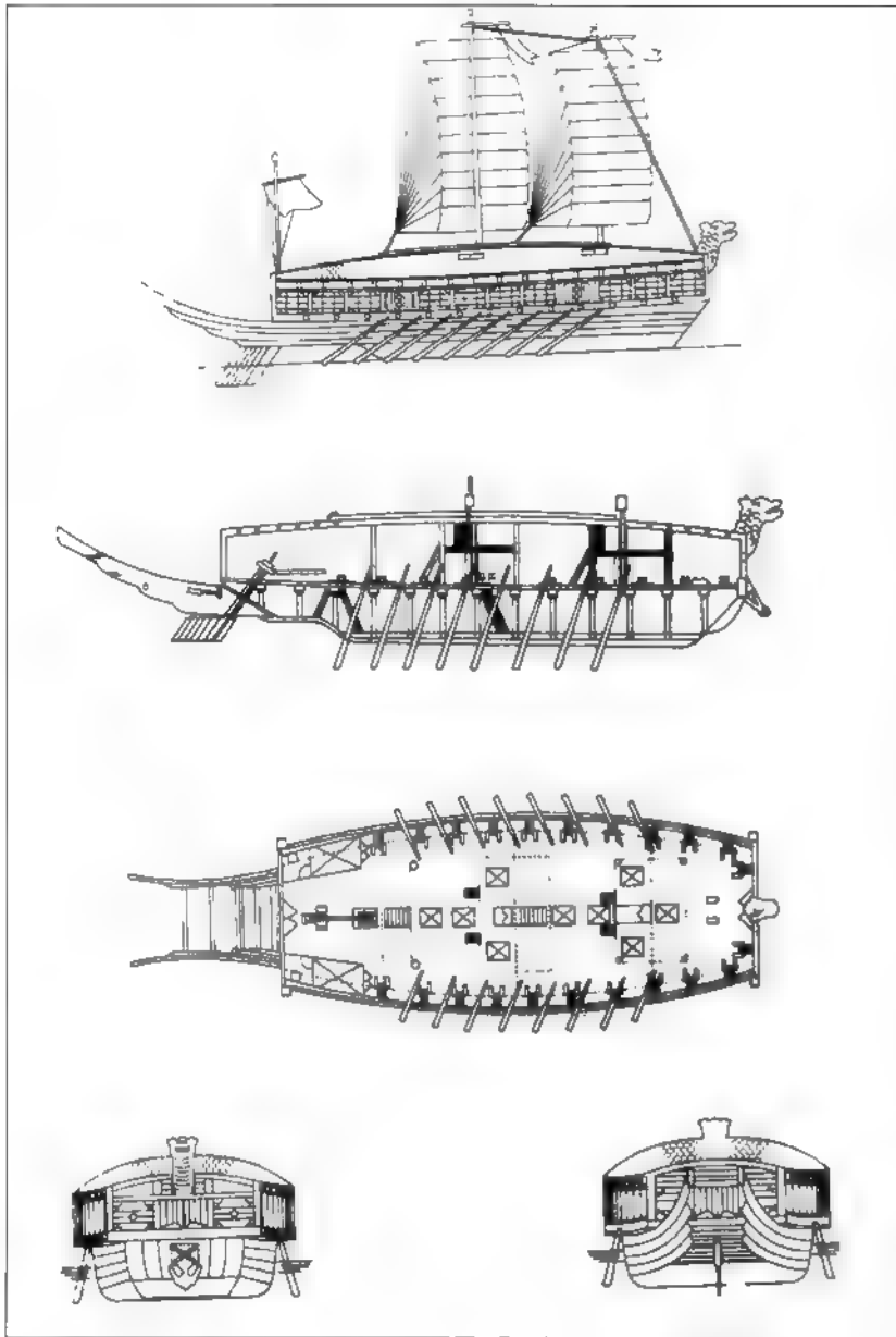
Plan, and side elevations of the turtle ship, based on the 1975 reconstruction drawings that have provided the basis for all reproductions since that date.
